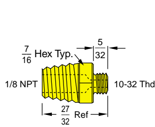
90 AN 1/8 to 10-32
