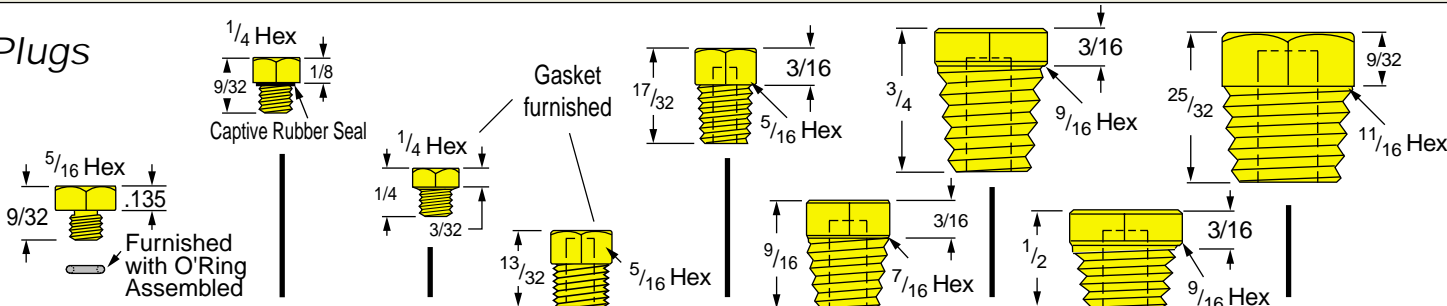
10-0 Plug
