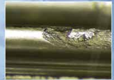
Macropitting/Spalling
